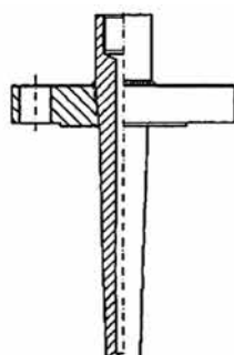
Barstock standard type.
