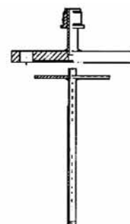
Two pieces for flange mounting. Wetted parts in: stainless steel 316, Hastelloy c276,c4, nickel, tantalum, zirconium, titanium.
