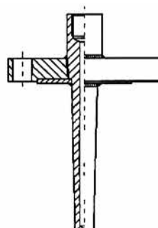
Barstock with rotating or welded flange. Wetted parts in: hastelloy c276,c4, nickel, titanium.
