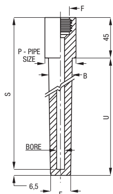
Socket weld
